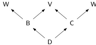
Figure 1 — Name lookup [fig:class.lookup]
