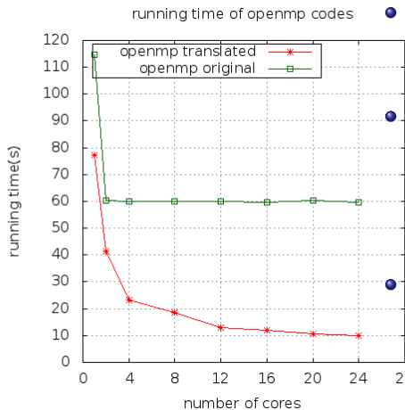
Figure: Mergesort: n = 5 \cdot 10^8
