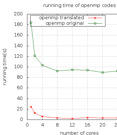
Figure: Matrix_inverse: n = 4096
