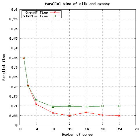
Figure: Linear system solving (dense method).
